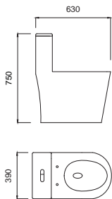
Super vortex siphon one-piece toilet LZ1234M/L
